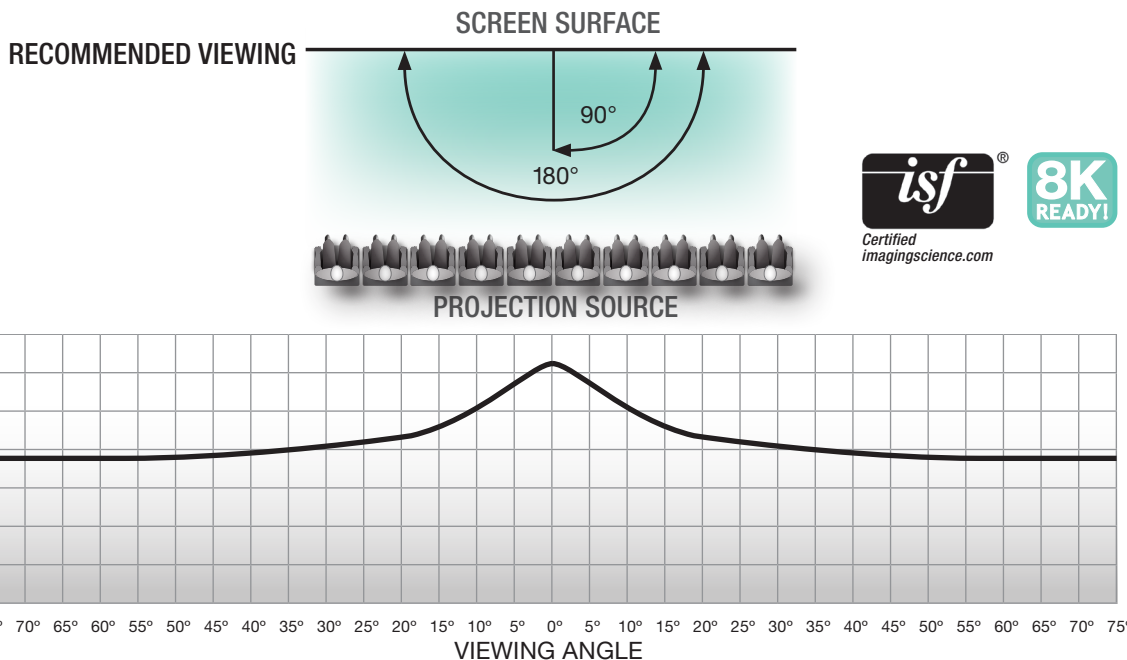
GAIN CHART TECVISION XT1600X WHITE
